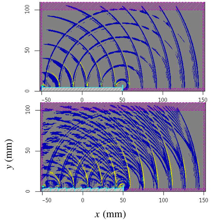
FIG. 8. (Color) B_z contour maps with a flat ground plane (upper) and with a grating (lower) (MIT).
