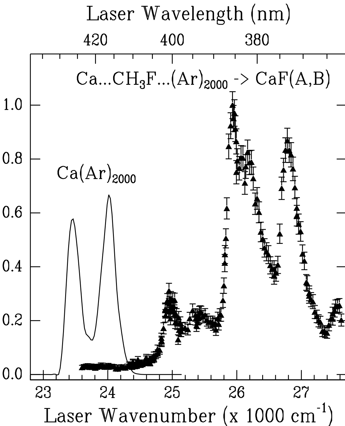
Figure 4: Action spectrum for the formation of the excited CaF product (experimental points). For comparison, the solid curve shows the excitation spectrum of the Ca( 4s4p^1P )Ar 2000 fluorescence when no CH 3 F molecule is present on the argon cluster.
