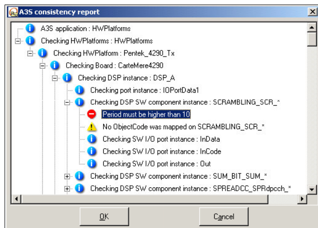
Fig. 2: Checking result of a SW application after deployment
