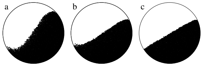
FIG. 4: Side-views of the 3D-drum. In all cases, R = 40 d , \mu = 0.3 , and \Omega=0.2 rad/s. a) L = 10 d , b) L = 50 d , c) L = 300 d . The longer the channel, the flatter the surface. This result gives further support to the idea that the end plates are responsible for the S shape of the free surface.
