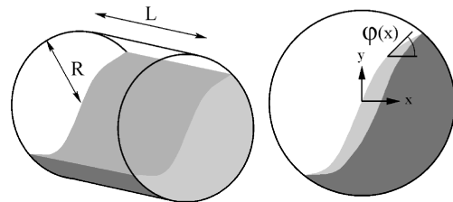
FIG. 1: We consider a half-filled three dimensional drum of radius R and length L . The local slope of the free surface is denoted \varphi(x) . Right: light grey corresponds to flowing material and dark grey to solid rotation.
