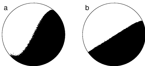
FIG. 2: Side views of the 3D drum. In both cases, R = 80d , L = 10d , \mu = 0.3 , \Omega=0.1 rad/s and N=36\,000 grains. a) frictional and b) frictionless end plates. The difference in shape is very clear and originates from a change in the frictional properties of the end plates. This provides evidence of the crucial role of the end plates on the shape of the free surface.
