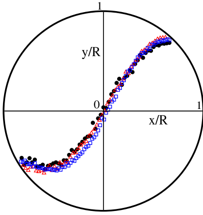
FIG. 5: (Color online) Rescaled plots of the position of the free surface for various values of R , L and \Omega : Triangles: R = 80d , L = 10d , \Omega = 0.05\text{rad/s} , Squares: R = 80d , L = 20d , \Omega = 0.2\text{rad/s} , Circles: R = 40d , L = 10d , \Omega = 0.2\text{rad/s} . In the simulation, the position of the free surface is calculated by identifying the highest grain located at a position x . R , L and \Omega are varied while keeping \Lambda constant. The data collapse onto one unique curve which validates the proposed scaling laws.
