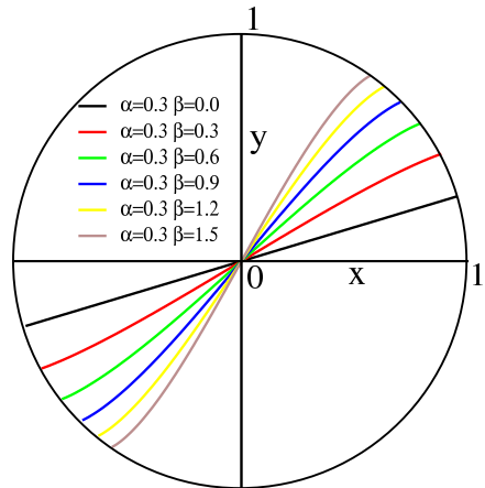
FIG. 3: (Color online) Numerical solutions for y_{surf} for R = 1 , \mu_i = \alpha = 0.3 and various values of \beta = \mu_w/L (d\Omega^2/g)^{1/4} . For \beta = 0 , the influence of the end plates is null and the free surface is flat. When \beta is increased, i.e. increasing influence of the end plates, a curvature appears and the free surface displays an S shape.
