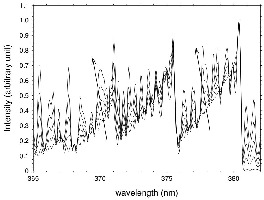
Figure 4 : Resulting Spectra (Schumann-Runge system of O 2 and second positive system of N 2 ) for several \chi^* (0.01, 0.20, 0.50, 1.00, 2.00) values versus wavelength. ( T_{rot}=2000 K, T_{vib}=4000 K, FWHM=0.19 nm).
