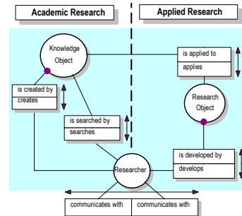
Fig. 2. Partial NIAM/ORM Model of the knowledge production and exchange processes in the Research UoD.
