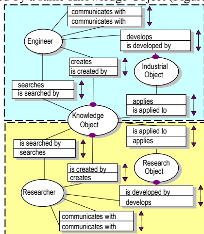
Fig. 4. Partial NIAM/ORM Model of the knowledge production and exchange processes in Research and Industrial UoDs.
