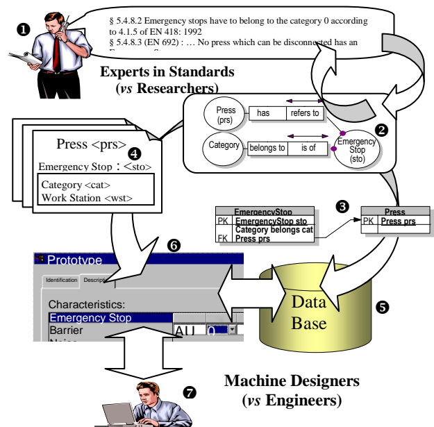
Fig. 9. Overview of the ACOMAS/CASA Method
