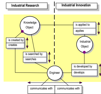
Fig. 3. Partial NIAM/ORM Model of the knowledge production and exchange processes in the Industrial UoD.
