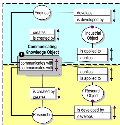
Fig. 8. "Communicating" Knowledge Object Model
