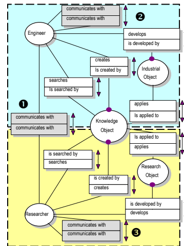
Fig. 5. Partial NIAM/ORM Model including direct communications between Researchers and Engineers
