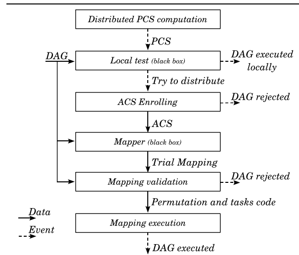
Figure 1. Algorithm overview
