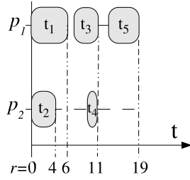
Figure 4. The schedule \mathcal{S}^* computed by the Mapper
