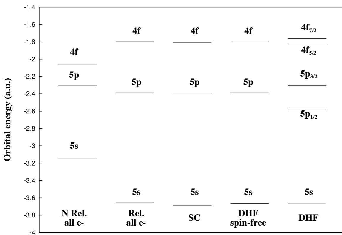
Figure 2: valence orbital energies for \text{La}^{3+} from various calculation levels
