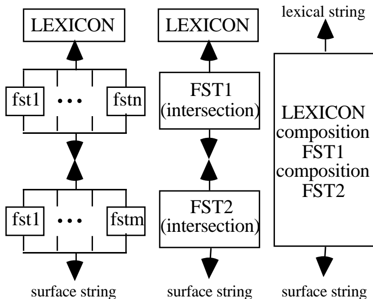
Fig. 7 Lexical transducers (from Karttunen et al., 92)
