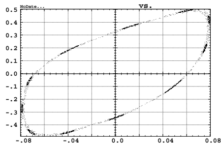
Figure 7: Effect of loss of precision in ITER. RK4 with 10 steps, so to insure good precision at all steps but the last step in ITER uses a \chi of one. Conclusion: spoiling the precision in the last step is enough to spoil the overall symplecticity, it decreases the precision of the integrator to an RK1 integrator.
