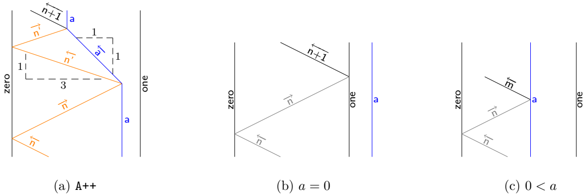
Figure 7: Implementations of A++ and n : \text{IF } A \neq 0 \text{ } m .
