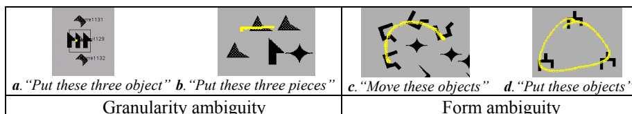
Fig. 7. Referring ambiguities
