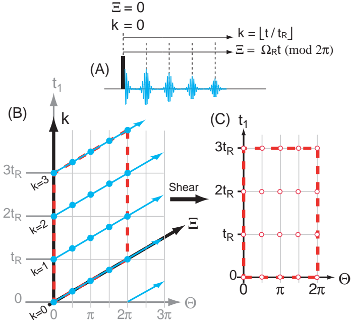
Fig. 1. (A) One pulse sample spinning experiment with coordinate definitions and timings. (B) Sampling trajectory (blue lines) of one pulse sample spinning data in the 2D t - \Theta and k - \Xi coordinate systems. The slope of the sampling trajectory in the t - \Theta coordinate system is the inverse rotor frequency. Identical data sets run parallel in the 2D plane and are separated by t_R and 2\pi , respectively, t - \Theta coordinate system. (C) Sheared 2D data set that correlates time and rotor pitch.
