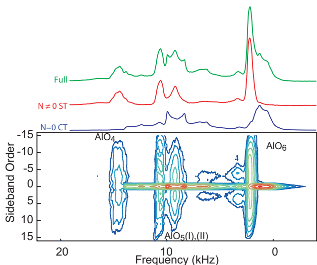
Fig. 4. ^{27}\text{Al} TOP spectrum, and projections of \text{A}_9\text{B}_2 ( 9\text{Al}_2\text{O}_3\text{-}2\text{B}_2\text{O}_3 ) acquired at 17.6 T with \Omega_R/2\pi = 31248 Hz (1 MHz spectral width, 1\mu\text{s} pulse \approx \pi/6 , 1s recycle time, 300 scans).
