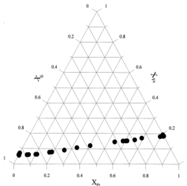
Fig. 9. Non-equilibrated Fe-Ir-Pt alloys and the effect of Pt/Ir on the Fe content of the alloys. The values of a_{\text{FeO}}^{\text{liq}} were calculated from the f\text{O}_2 and the composition of Ir-Fe binary (left, a_{\text{FeO}}^{\text{liq}} = 0.081 ) and Pt-Fe binary (right, a_{\text{FeO}}^{\text{liq}} = 0.077 ). See Table 3 and text (5.1.3).
