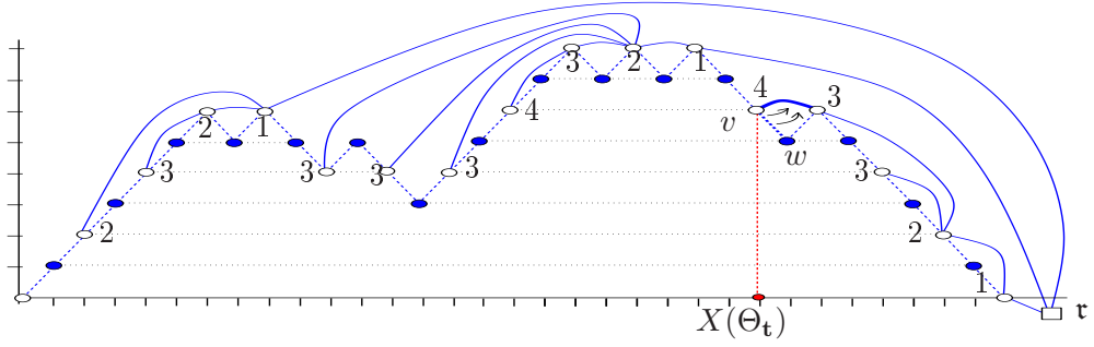
Figure 6: Drawing \mathcal{D} on \mathcal{G} .
