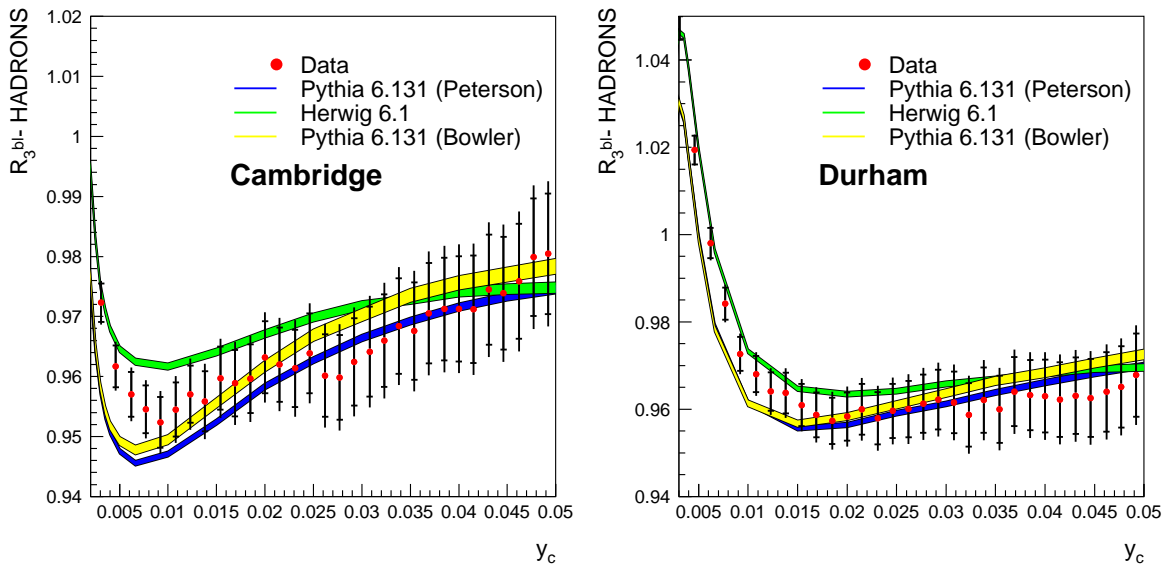
Figure 7: R_3^{b\ell} at hadron level as a function of y_c compared with PYTHIA 6.131 (with Peterson and Bowler fragmentation b functions) and HERWIG 6.1 predictions, using the CAMBRIDGE (left) and DURHAM (right) jet-clustering algorithms.
