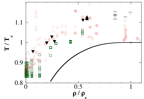
FIG. 1: Phase diagram of {}^4\text{He} in reduced units ( T_c = 5.1953 K, \rho_c = 69.641 \text{kgm}^{-3} ) showing the location of various measurements of Nu versus Ra . Solid line: coexistence curve. Asterisk: critical point. Open diamonds: Niemela et al. [9]. Open squares: Wu et al. [7, 8]. Triangles up and down: Chavanne et al. [4]; triangles up: \beta\Delta T < 0.1 , triangles down: \beta\Delta T > 0.1 , open: near the critical isochore, solid: far from the critical isochore.
