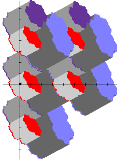
Figure 2: Tiling of \mathbb{R}^3 for the Tribonacci expansion
