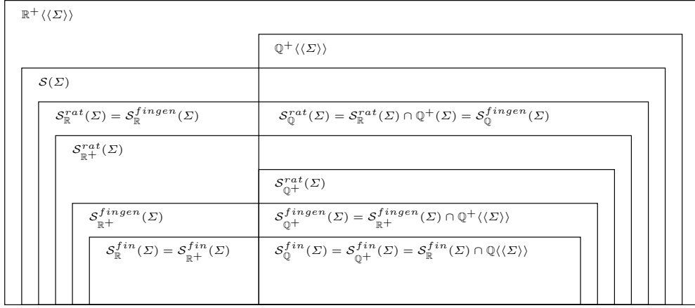
Fig. 6. Inclusion relations between classes of classes of rational stochastic languages, including \mathcal{S}_K^{ingen}(\Sigma) and \mathcal{S}_K^{in}(\Sigma) .
