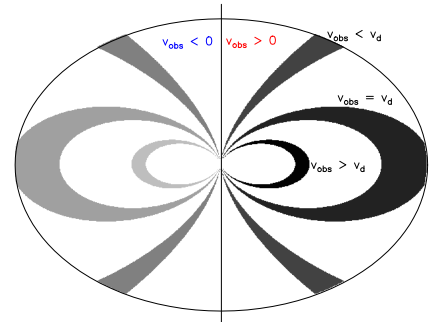
Fig. 2. Regions of the disk which yield equal projected velocities v_{\text{obs}} . The outer ellipse is the projection of the disk outer edge.
