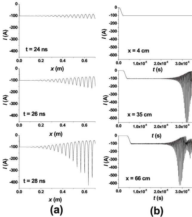
FIG. 6. (a) Current as a function of x at three different times. (b) Current as a function of time at three different locations along the grating.
