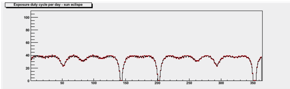
Figure 10 : The day averaged duty cycle in percent (fraction of active time during one day) for one year if one only takes the sun into account.
