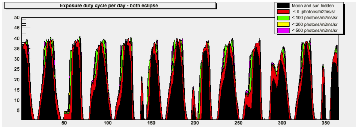
Figure 14: The day averaged duty cycle for one year asking the sun and the moon to be hidden (both \theta_{zenith} > 109.18^\circ , in black), and accepting increasing amount of moonlight induced background (0 or quasi-null, 100, 200 and 500 photons/m 2 /ns/sr).
