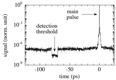
FIG. 1: Laser pulse temporal contrast measured with a third order autocorrelator (logarithmic scale). The detection threshold was determined blocking the laser beam during the scan between 80 and 70 ps before the main pulse.
