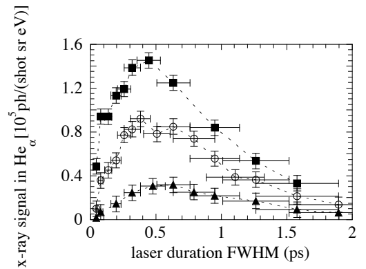
FIG. 8: X-ray emission in the \text{He}_\alpha line measured from clusters with 275 Å average radius, as a function of the laser duration. Full triangles : 1.8 mJ in the laser pulse corresponding to a maximum fluence of 4.8 \times 10^3 \text{ J/cm}^2 . Empty circles : 2.8 mJ, i.e. 7.5 \times 10^3 \text{ J/cm}^2 . Full squares : 3.8 mJ, i.e. 1.0 \times 10^4 \text{ J/cm}^2 .
