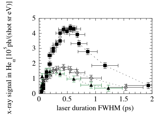
FIG. 7: X-ray emission in the \text{He}_\alpha line measured as a function of the laser duration. Ar clusters with different sizes are irradiated by 3.0 mJ laser pulses, i.e. a maximum fluence on target of 8.0 \times 10^3 \text{ J/cm}^2 . Full triangles : clusters with 180 Å average radius are irradiated. Empty circles : 275 Å. Full squares : 350 Å.
