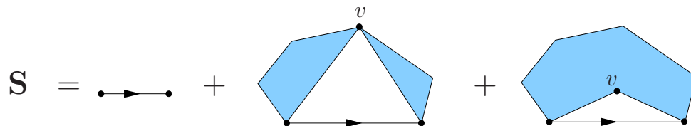
FIGURE 4. Decomposition of non-separable near-triangulations.
