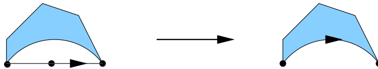
FIGURE 9. A bijection between \mathbf{W}_2 and \mathbf{W} .
