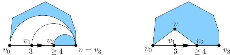
FIGURE 18. Two configurations for a map in \mathbf{V}_{3, \geq 4} .
