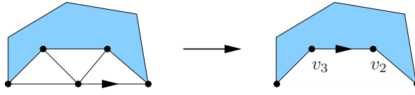
FIGURE 14. A bijection between maps of the third type in \mathbf{V}_4 and \mathbf{V}_{\geq 4, \geq 4} .
