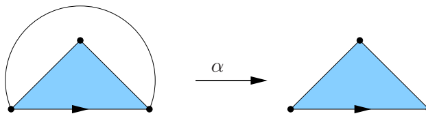
FIGURE 3. Near-triangulations rooted on a digon and triangulations.
