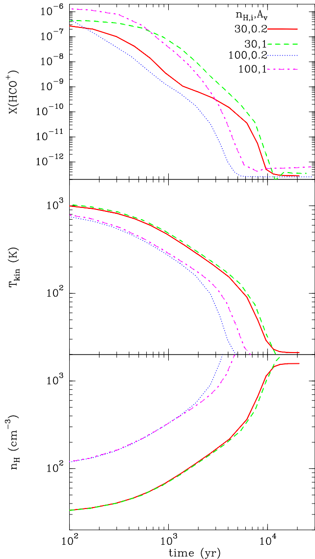
Fig. 10. Time-dependent evolution of ( top ) the HCO + abundance, ( middle ) the kinetic temperature and ( bottom ) the hydrogen density, along the isobaric cooling of a parcel of gas formerly enriched chemically in a burst of dissipation of turbulent energy. The initial densities are n_{H,i} = 30 (dashed and solid) and 100 \text{ cm}^{-3} (dotted and dot-dashed), and the shieldings from ISRF are A_V = 0.2 (solid and dotted) and 1 mag (dashed and dot-dashed)
