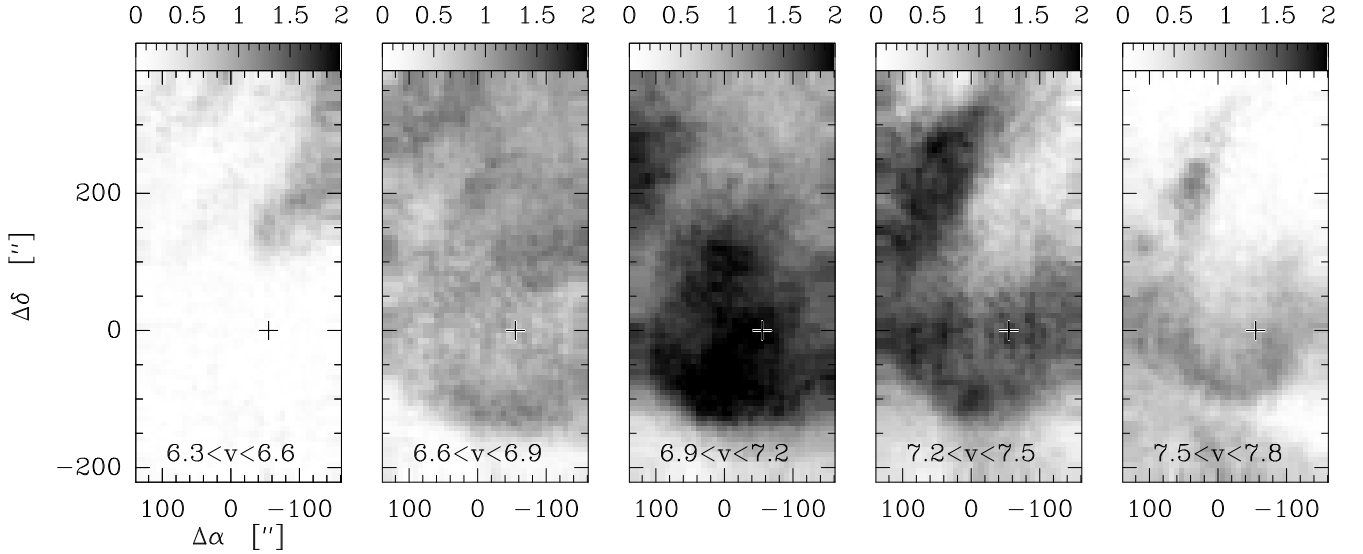
Fig. 2. ^{12}\text{CO}(J=2-1) channel maps of the L1512 field. The position observed in HCO + is at offset (-55'', 0) relative to (0,0) : RA=05h00m54.5s, Dec=32° 39' (1950). The dense core is centered on the (0,0) position and is about 2 arcmin in diameter (Lee, Myers & Tafalla 2001, Pety & Falgarone (2003)). The velocity intervals in \text{km s}^{-1} are given at the bottom of each panel.
