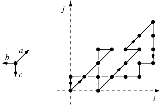
Figure 1: Kreweras' walks in a quadrant.
