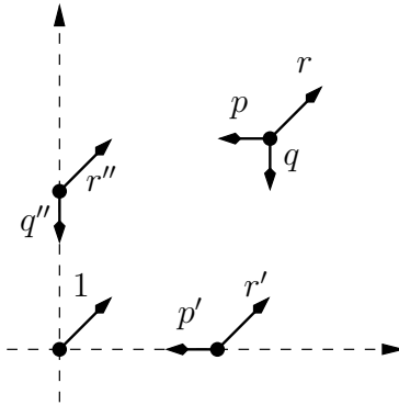
Figure 3: The transition probabilities.
