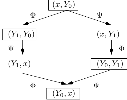
Figure 2: The orbit of (x, Y_0) under the action of \Phi and \Psi . The framed pairs can be substituted for (x, y) in the functional equation.
