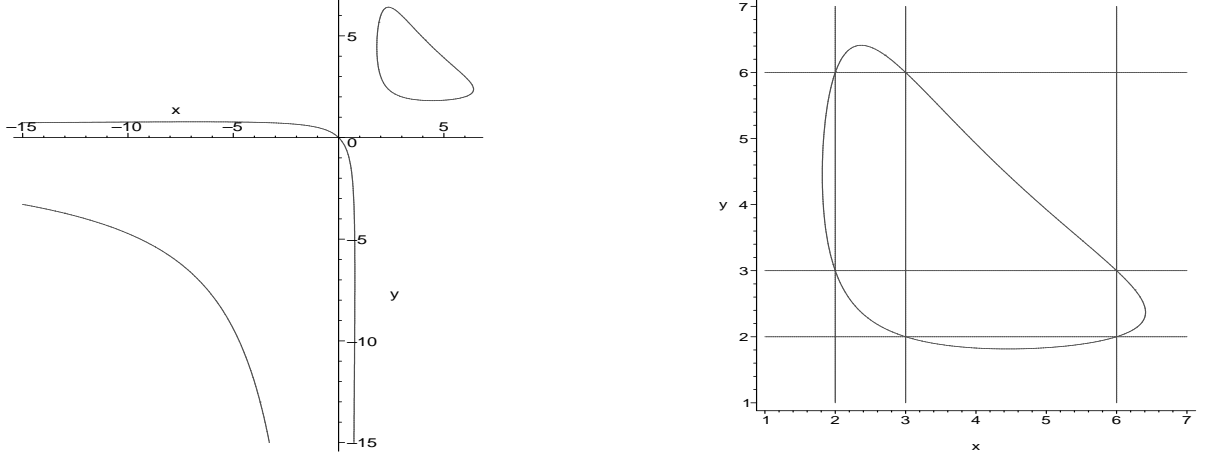
Figure 4: The real branches of the functions Y_i , for p = 1/3, q = 1/2 and r = 1/6 .
