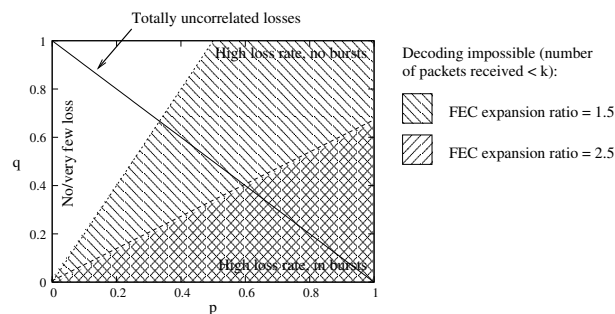
Figure 9.4: Loss limits.
