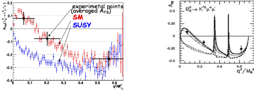
Figure 2: (Left) Forward-backward asymmetry for \Lambda_b \rightarrow \Lambda \mu^+ \mu^- decay [6]. (Right) Forward-backward asymmetry for B_d^0 \rightarrow K^* \mu^+ \mu^- decay [7].
