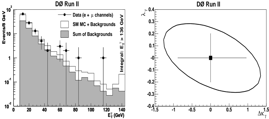
FIGURE 8. D\bar{O} : The photon E_T spectrum (on the left) for the W\gamma candidates with M_T(W,\gamma) > 90 GeV/ c^2 . The points with error bars are the data and the open histogram is the sum of the SM Monte Carlo prediction and background estimate. On the right: limits on the WW\gamma TGC \Delta\kappa_\gamma and \lambda_\gamma . The points indicate the SM value with the error bars showing the 95% C.L. intervals in one dimension. The ellipse represents the two-dimensional 95% C.L. exclusion contour.
