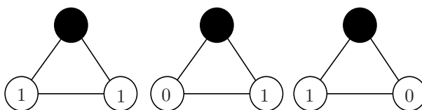
Figure 2: Recurrent configurations on C_3 .
