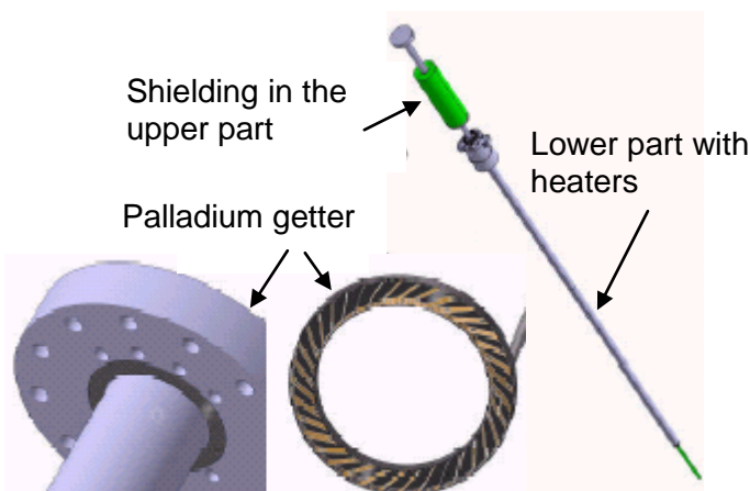
Figure 11: Central rod with the palladium getter for absorbing Hg vapours in the cover gas.
