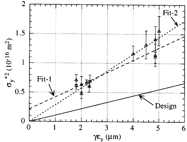
Figure 4. Vertical spot size (squared) versus the incoming vertical emittance. Measured in September 1994 with the Laser-Compton monitor. Fit-1 (dashed) is the linear fit to the measured data, Fit-2 (dotted) is the linear fit passing the origin, and the solid is the design line.
