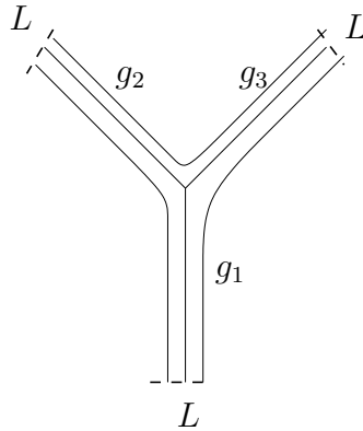
FIGURE 6. G' consisting of three periodic loops, \{g_1, g_2\} , \{g_2, g_3\} , and \{g_3, g_1\} .
