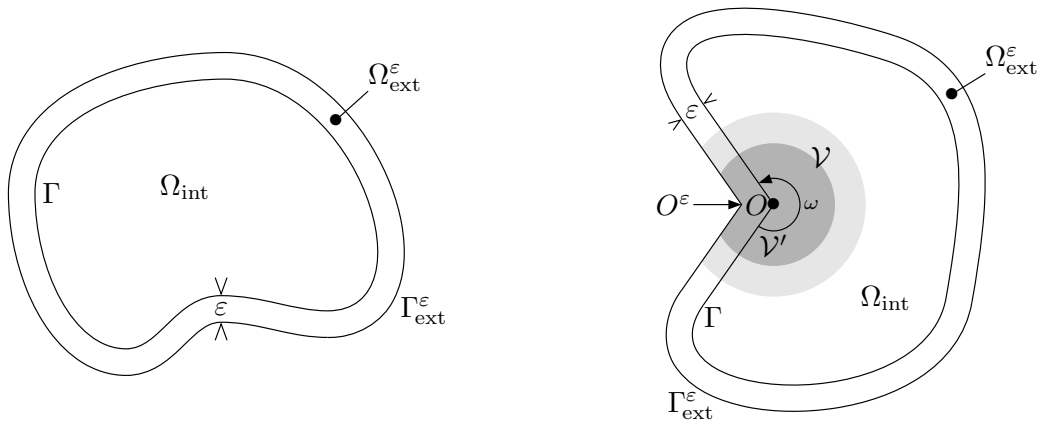
Figure 1: The smooth and corner domains with thin layer \Omega^\varepsilon .
