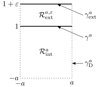
Figure 5: The rectangle \mathcal{R}^{a, \epsilon} .
