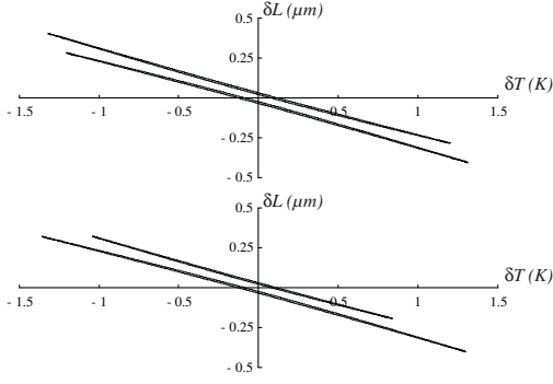
Fig. 7. Locking zone as a function of cavity length and crystal temperature for two values of \xi : top \xi = 0 , bottom \xi = \pi/4 . The other values are the same : \rho = 5^\circ , \sigma = 3 .
