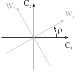
Fig. 1. \rho is the angle between the crystal's axes ( (C_1, C_2) , black lines) and the waveplate axes ( (W_1, W_2) , grey lines).
