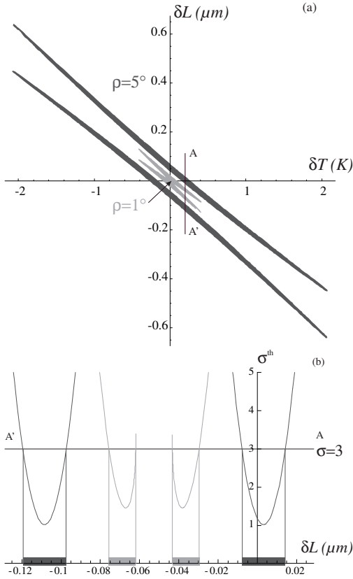
Fig. 3. (a) : Locking zone as a function of the cavity length ( \delta L ) and of the crystal temperature ( \delta T ) for waveplate angle \rho = 1^\circ (light grey) and \rho = 5^\circ (dark grey). \sigma = 3 . (b) : \sigma^{th} as a function of the cavity length ( \delta L ) for \delta T = 0.2 K . For \sigma = 3 , this corresponds to the cross section AA' of the locking zone. \Delta\phi = \pi .
