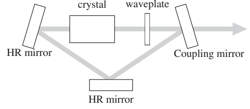
Fig. 2. Set-up of the ring cavity; we consider only one direction of propagation.
