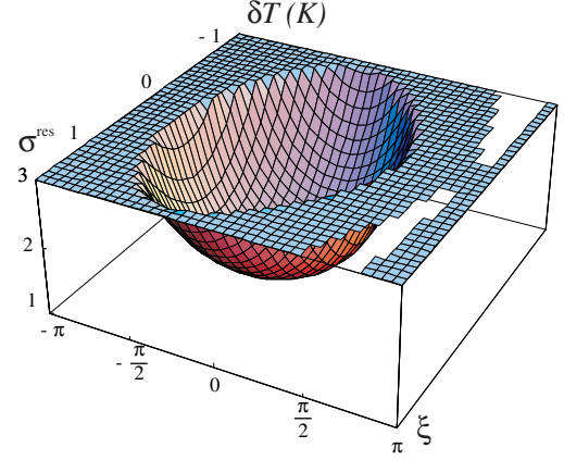
Fig. 8. Normalized threshold on resonance \sigma_{res} as a function of the crystal temperature \delta T and of the phase-shift \xi for \rho = 5^\circ . Unshaded surfaces correspond to values of (\delta T, \delta L) where frequency degenerate operation is not possible.
