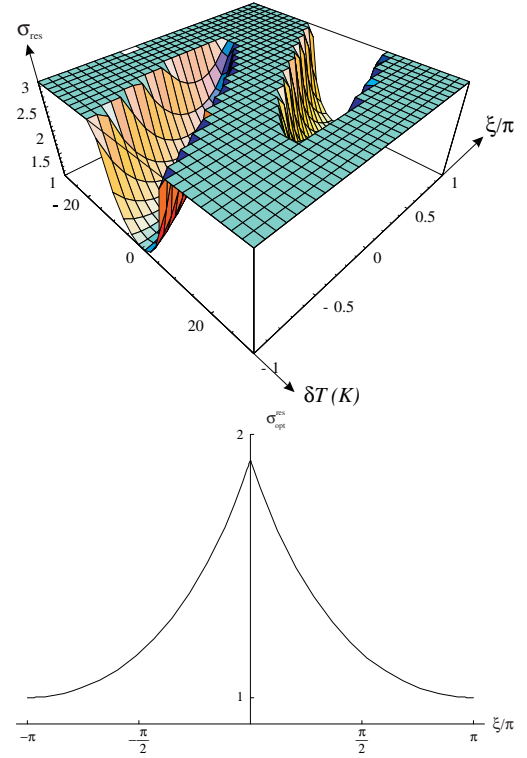
Fig. 9. Normalized threshold on resonance \sigma_{res} as a function of the crystal temperature \delta T and of the phase-shift \xi for \rho = 45^\circ (top). Same curve optimized for \delta T (bottom)
