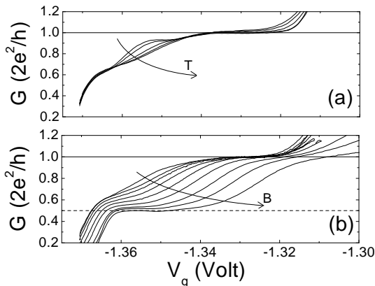
FIG. 1: a) Conductance characteristics G(V_g) at T = 273, 360, 515, 666 and 779 mK. With increasing temperature the resonance at 0.9 \times 2G_0 disappears, whereas the 0.7 structure (in this case close to 0.65 \times 2G_0 ) becomes more pronounced. (b) G(V_g) at T = 560 mK in parallel fields B = 0 to 8 Tesla, in steps of 1 Tesla. With increasing B , the 0.7 structure evolves into the spin-split plateau at G_0 .
