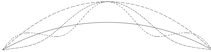
Fig. A.3. Deformations of a spherical cap of radius 1 and half-angle \pi/6 . The deformations are due to Legendre functions P_{y_l} . For clarity, the maximum amplitude of the deformation is fixed to 0.1. This value is too large in principle for the linear analysis. The solid curve is the initial state. The largest dashed is the case l = 0 . The intermediate dashed is the case l = 1 . The smallest dashed is the case l = 2 .
