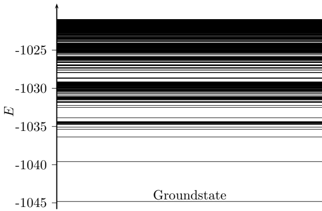
FIG. 2: Lowest energy levels for q = 5, \sigma = 0.5, N = 400 , computed by sorting energy samples from a long simulation run. Each level is drawn as a horizontal line.
