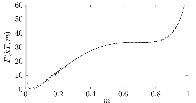
FIG. 10: Partial free energy F(kT, m) for q = 9, \sigma = 0.3, L = 400 (solid line), together with the MF prediction (dashed line) as given by Eq. (1).
