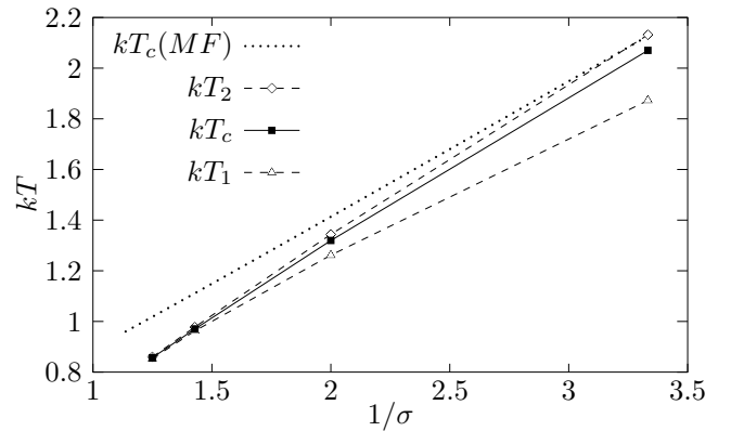
FIG. 9: Spinodal curve for 0.3 \leq \sigma \leq 0.8 ( q = 5 ). The transition temperature T_c is indicated by filled squares, and the limits of metastability T_1 and T_2 by triangles and diamonds, respectively. Errors are smaller than the size of symbols, and lines are drawn to guide the eyes. The dotted line shows the transition temperature as predicted by MF theory.
