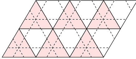
FIG. 3: The lattice of Potts spins is shown in solid linestyle. There are two-spin interactions along every edge, and three-spin interactions among the spins surrounding the up-pointing faces (shaded). The loop model is defined on a shifted triangular lattice, shown in dashed linestyle.
