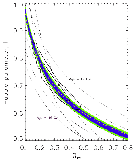
Figure 1: Constraints set by the properties of the first peak as seen by WMAP in the \Omega_m - h plane for a flat universe (filled region, blue, 1 \sigma , green 2 \sigma ). The constraint region follows almost exactly constant age lines (dotted). Additional constraints can be obtained on the dark matter content for powerlaw CDM models (dashed lines), leading to tight contours when combined. From Page et al. (2003).
