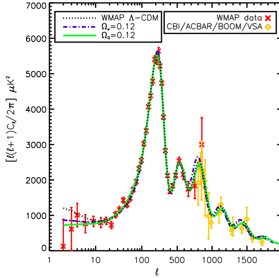
Figure 2: The temperature power spectrum for the best-fit power-law \Lambda CDM model (dotted black line) from Spergel et al. (2003), and for two broken-power-law models (both having \Omega_\Lambda = 0 ) with \Omega_\nu = 0.12 (dot-dashed blue line) and \Omega_Q = 0.12 (solid green line), compared to data from WMAP and other experiments ([10, 31, 20, 33]). Such models have a low Hubble constant ( H_0 \sim 46 km/s/Mpc) and of course are rejected by the interpretation of the SNIa Hubble diagram but are consistent with most major cosmological data (large scale structure, abundance of local clusters, dark matter distribution on large scales as observed from weak lensing, primordial nucleosynthesis). From Blanchard et al. (2003)
