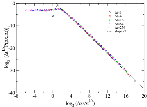
FIG. 5: After rescaling the distribution of ultrametric distances d_u between sites depinning at time t and t+\Delta t collapse on a unique master curve. The dynamic exponent used for the rescaling is z = 1.39 .
