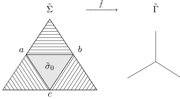
Figure 4: Fibers of \tilde{f}
