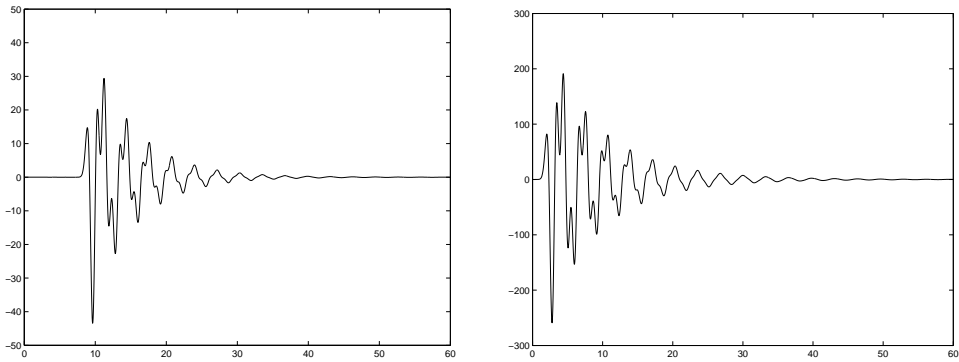
Figure 7.15: Temporal records of ground response in Mexico City-like environment for various very large (left panel: \mathbf{x}^s = (0\text{m}, 3000\text{m}) , \mathbf{x} = (3000\text{m}, 0\text{m}) ) and very small (right panel: \mathbf{x}^s = (0\text{m}, 100\text{m}) , \mathbf{x} = (100\text{m}, 0\text{m}) ) source-to-observation point distances).
