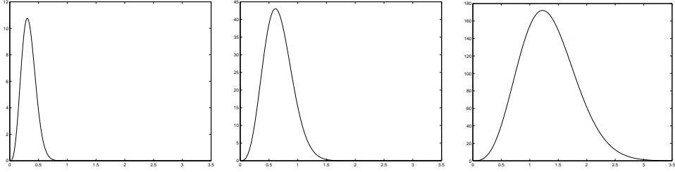
Figure 7.1: Moduli of source spectrum functions, i.e. |S(\nu = \omega/2\pi)| versus \nu (Hz), for \nu_0 = 0.25 Hz (left), 0.50Hz (middle), 1.0Hz (right).
