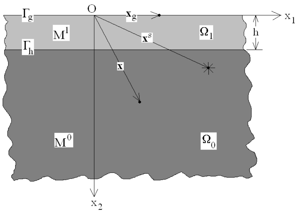
Figure 2.1: Cross section view of the configuration.
