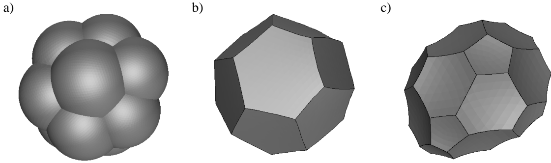
Figure 1: Examples of the clusters considered here with V_c = V = 1 in each case: (a) cluster of F = 13 outer bubbles (that is, a total of F + 1 = 14 bubbles) still attached; (b) the central bubble, drawn to a different scale, with F = 13 faces (this is a Matzke cell [22] with one square, ten pentagonal and two hexagonal faces); (c) a bubble with F = 26 faces (all pentagonal or hexagonal) – note its departure from approximate sphericity, described in §3.2.
