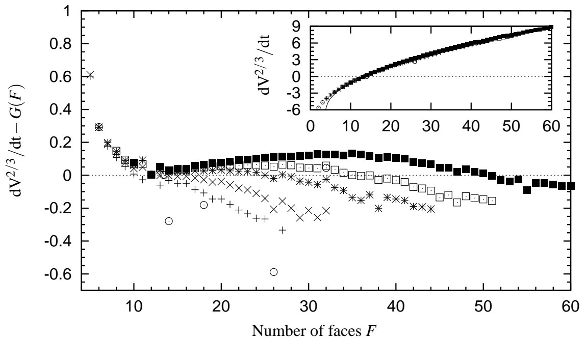
Figure 7: The difference in the rate of change of volume of a bubble with F faces, calculated from our simulations using (1), and the value calculated according to the analytic formula (2). The inset shows the values themselves, again next to the analytic line, from which it deviates at small F . Data is shown for volume ratios of V_c/V = \frac{1}{2}(+), 1(\times), 2(*), 3(\square) and 5(\blacksquare) . The data for bubbles with constant curvature ( \odot ) [12], rather than fixed volume, is more scattered, but useful for low F .
