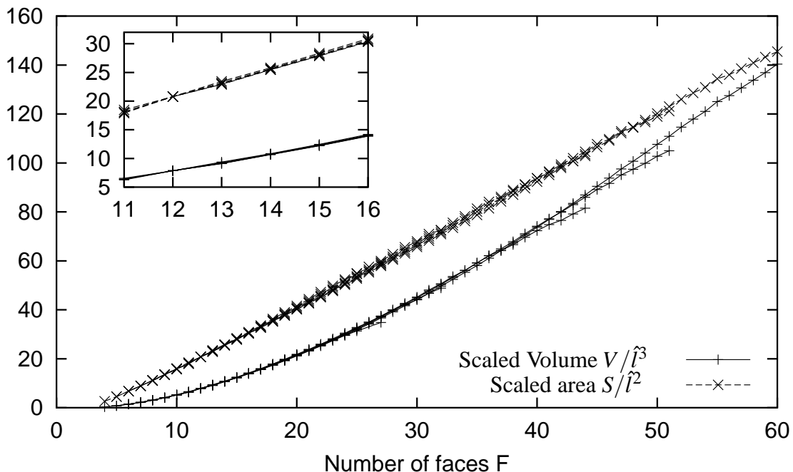
Figure 6: The volume V and surface area S of a bubble with F faces scaled with the average length of an edge \hat{l} . The data for the surface area is affine, S/\hat{l}^2 = 2.573F - 9.801 , while for low F the volume data is approximately quadratic, V/\hat{l}^3 \approx 0.053F^2 . Data is shown for all volume ratios V_c/V considered here, and the inset shows details of V and S for bubbles with 11 to 16 faces.
