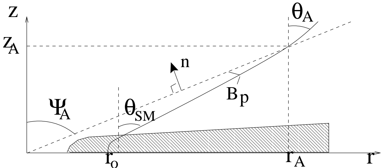
Fig. 1.— Geometry of a disk wind configuration and definitions of quantities related to the Alfvén critical surface. The unit vector \mathbf{n} is defined as (\mathbf{z}, \mathbf{r})/\sqrt{r^2 + z^2} .
