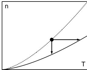
Figure 3: Critical line in the density-temperature plane, for the ideal gas (upper line) and for the interacting gas (lower line). Starting from a point on the first critical line, arrows indicate how a change of density at constant temperature, or conversely, move the point to the new line, as discussed in the text.
