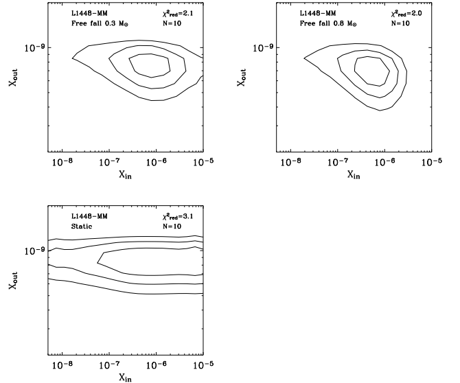
Fig. 9. \chi_{\text{red}}^2 diagrams of L1448-MM for three different velocity profiles. The upper left and upper right panels show the \chi_{\text{red}}^2 contours derived for a free falling envelope with a central mass of 0.3 and 0.8 M ⊙ respectively. The lower panel shows the static envelope case, with a 1 km s -1 turbulent velocity. Contours indicate the 1, 2 and 3 \sigma confidence levels respectively.
