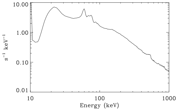
Fig. 10. ISGRI background spectrum observed while INTEGRAL was pointing to an empty field.
