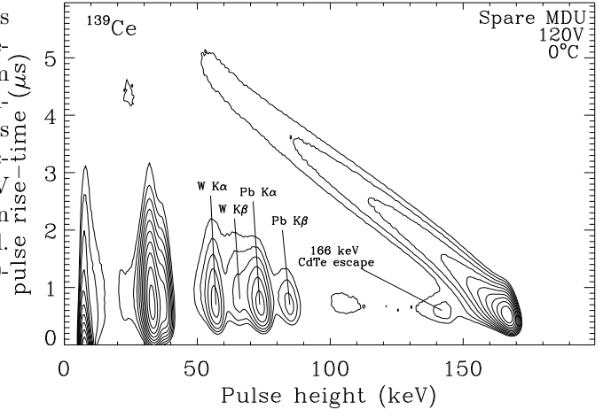
Fig. 4. Contour plot of the count per pulse-height and pulse rise-time bins.
