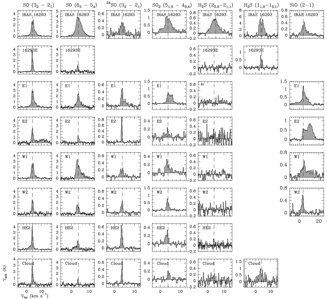
Fig. 3. Spectra (not smoothed) of \text{SO } 3_2 \rightarrow 2_1 \text{SO } 6_5 \rightarrow 5_4 ^{34}\text{SO } 3_2 \rightarrow 2_1 \text{SO}_2 5_{1,5} \rightarrow 4_{0,4} \text{H}_2\text{S } 2_{2,0} \rightarrow 2_{1,1} \text{H}_2\text{S } 1_{1,0} \rightarrow 1_{0,1} and \text{SiO } 2 \rightarrow 1 at “key” points (see text) in the L1689N molecular cloud. The vertical dashed line on each spectrum shows the position of the cloud systemic velocity ( v_{\text{LSR}}=3.9 \text{ km s}^{-1} ).
