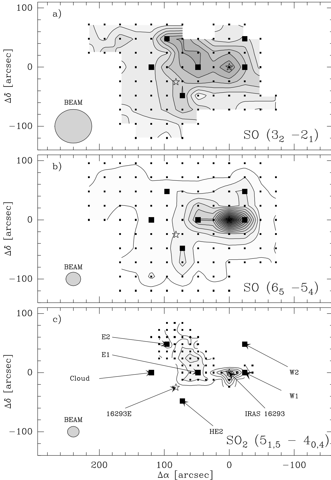
Fig. 2. Integrated intensity maps of \text{SO } 3_2 \rightarrow 2_1 (a), \text{SO } 6_5 \rightarrow 5_4 (b) and \text{SO}_2 5_{1,5} \rightarrow 4_{0,4} (c). (a) and (b) : first level is 0.5 \text{ K km s}^{-1} with level step of 1.0 \text{ K km s}^{-1} . (c) : first level is 0.3 \text{ K km s}^{-1} with level step of 1.0 \text{ K km s}^{-1} . In each map, the black points represent the observed positions. The two stars symbols show the position of the two protostellar sources. The arrows point to the eight “key” positions, whose spectra are displayed in Fig. 3.
