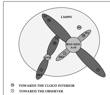
Fig. 1. Sketch of the region seen face on. The dark grey outflows have been clearly identified by CCLCL01. Light gray used for the outflow emanating from IRAS16293 and the W2 source indicates that these are only assumptions.
