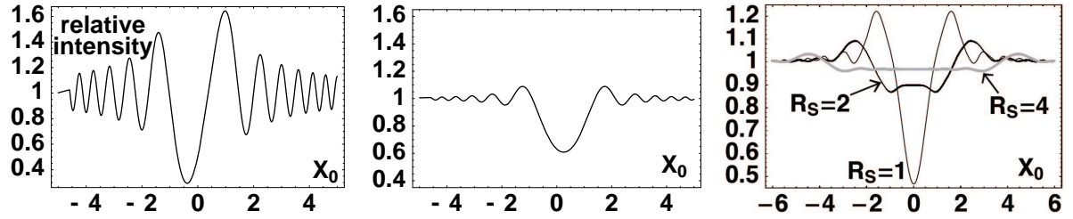
Figure 1: Relative intensity diffraction patterns produced in the observer's plane, perpendicularly to a width step or prism. From left to right: - Step of optical path \delta = \lambda/4 - Prism of optical path with \delta = X_0 \times \lambda/2 for X_0 > 0 . - Step of optical path \delta = \lambda/2 , for extended disk-sources of reduced radius R_S = 1, 2 and 4 . The X_0 - axis origin ( X_0 = x_0/\sqrt{\pi}R_F ) is the intercept of the source-step line with the observer's plane.
