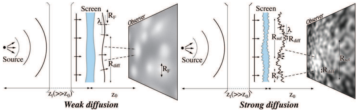
Figure 2: The two scintillation regimes: Left: R_{diff} \gg R_F . The weakly distorted wavefront produces a weak scintillation at scale R_F in the observer's plane. Right: R_{diff} \ll R_F . The strongly distorted wavefront produces strong scintillation at scales R_{diff} (diffractive mode) and R_{ref} (refractive mode).
